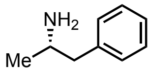
Dextroamphetamine
