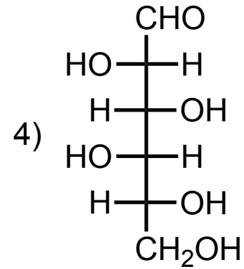
Iodose
