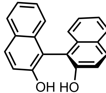
1,1'-Bi-2-naphthol (BINOL)
