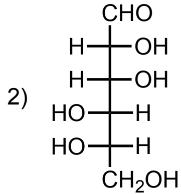
Mannose
