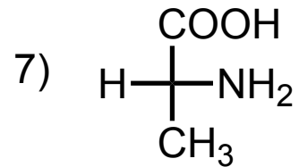
Alanine
