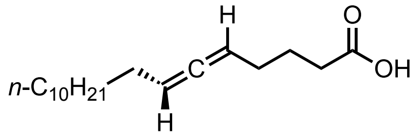
laballenic acid
