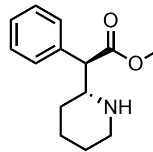
Dexmethylphenidate
