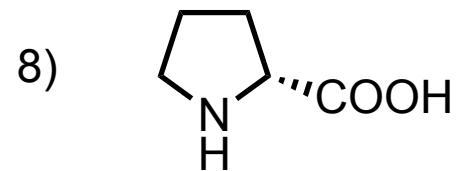
Proline
