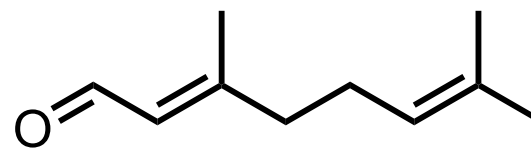
citral
