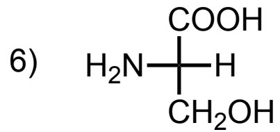
Serine
